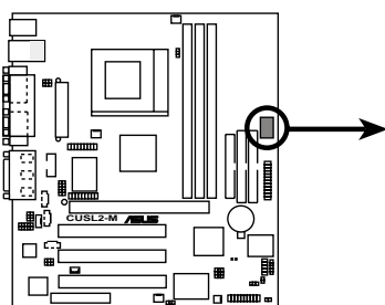
CUSL2-M DIP Switches
