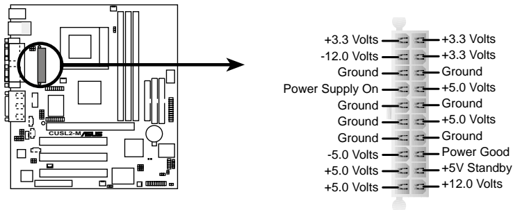
CUSL2-M ATX Power Connector
