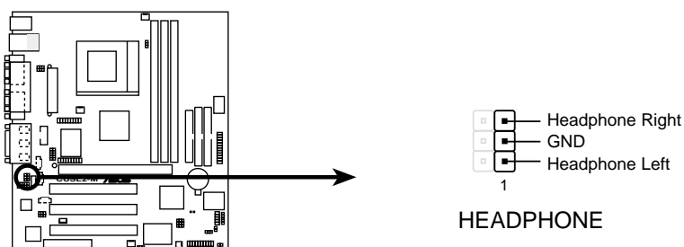
CUSL2-M True-Level Line Out Header
