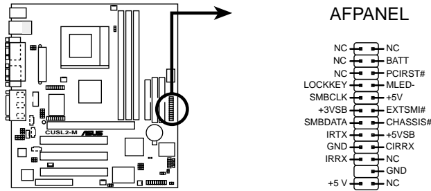
CUSL2-M Front Panel Connectors
