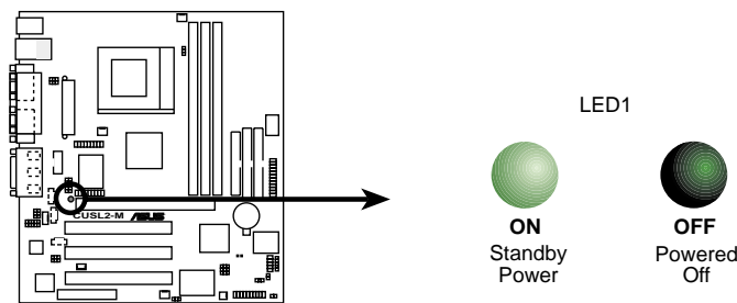
CUSL2-M Onboard LED
