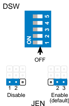
CUSL2-M JumperFree™ Mode Setting
