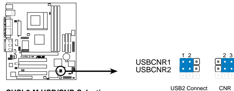
CUSL2-M USB/CNR Selection
