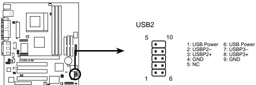
CUSL2-M USB Headers
