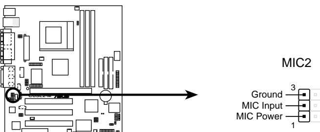
CUSL2-M Internal Microphone Connector
