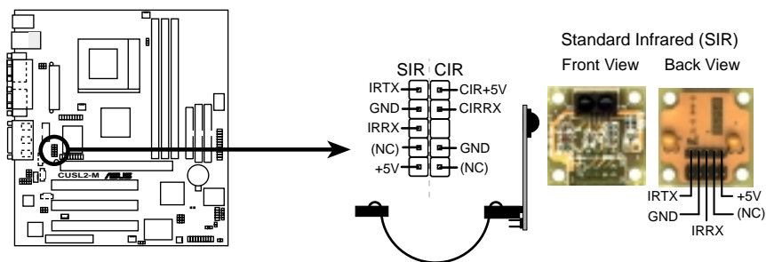
CUSL2-M Infrared Module Connector
