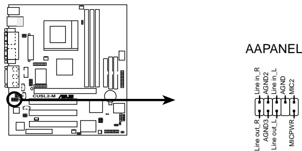
CUSL2-M Audio Panel Connectors
