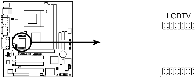
CUSL2-M LCD-TV Headers
