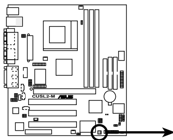
CUSL2-M Wake-On-Ring Connector
