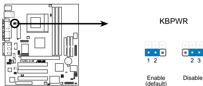
CUSL2-M Keyboard Power Setting
