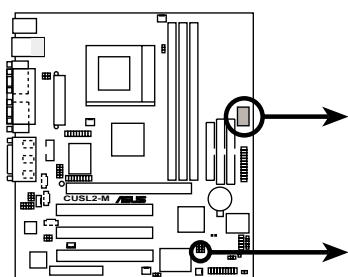
CUSL2-M JumperFree™ Mode Setting
