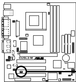
CUSL2-M Wake-On-LAN Connector
