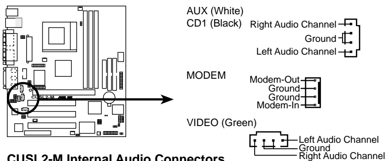
CUSL2-M Internal Audio Connectors
