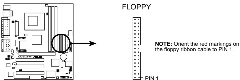
CUSL2-M Floppy Disk Drive Connector
