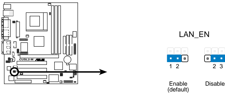
CUSL2-M On Board Lan Setting
