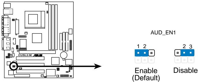
CUSL2-M Audio Codec Setting
