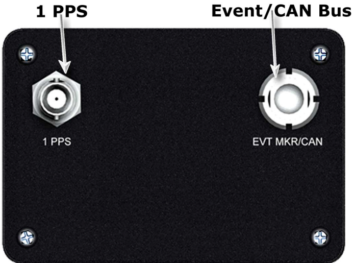
Figure 3: SF-2050M Only Back View
