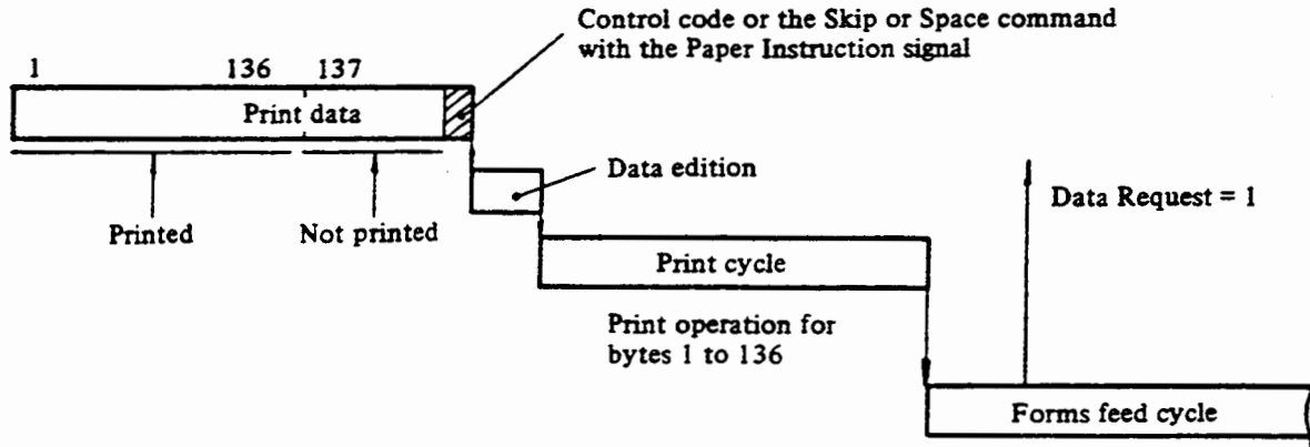
Figure 4.2 Print operation
