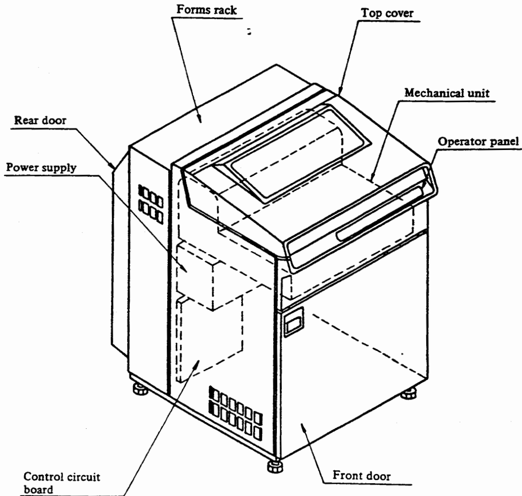
Figure 3.1 Printer configuration
