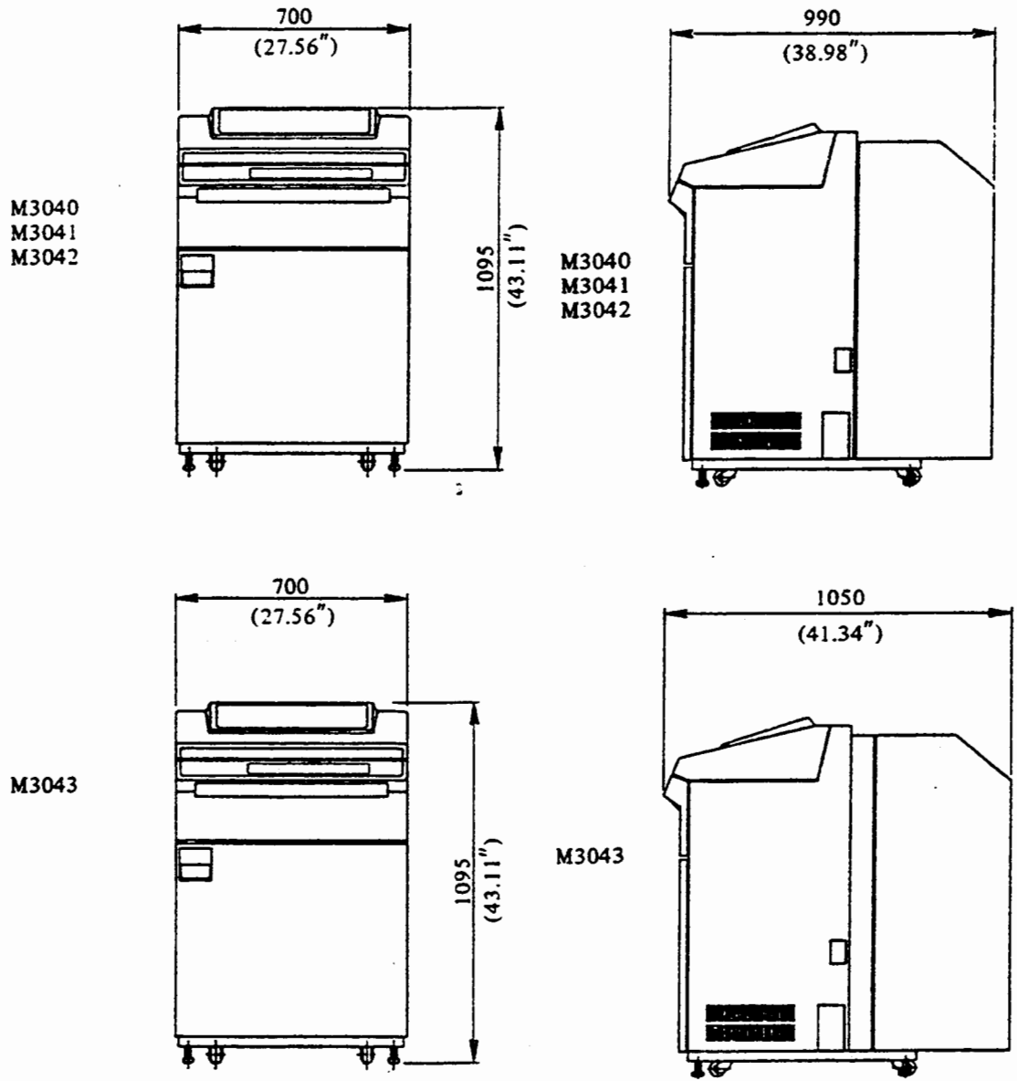
Figure 2.3 Outer dimensions (with the powered stacker)
