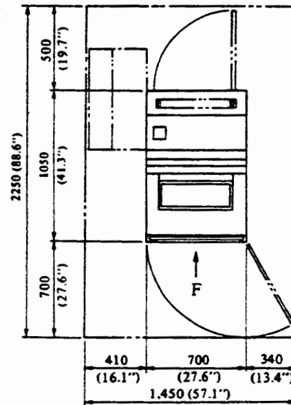
Figure 2.4 Operation and maintenance areas (with the powered stacker)
