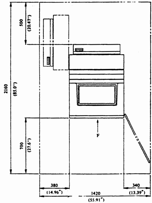
Figure 2.2 Operation and maintenance area (with the forms rack)
