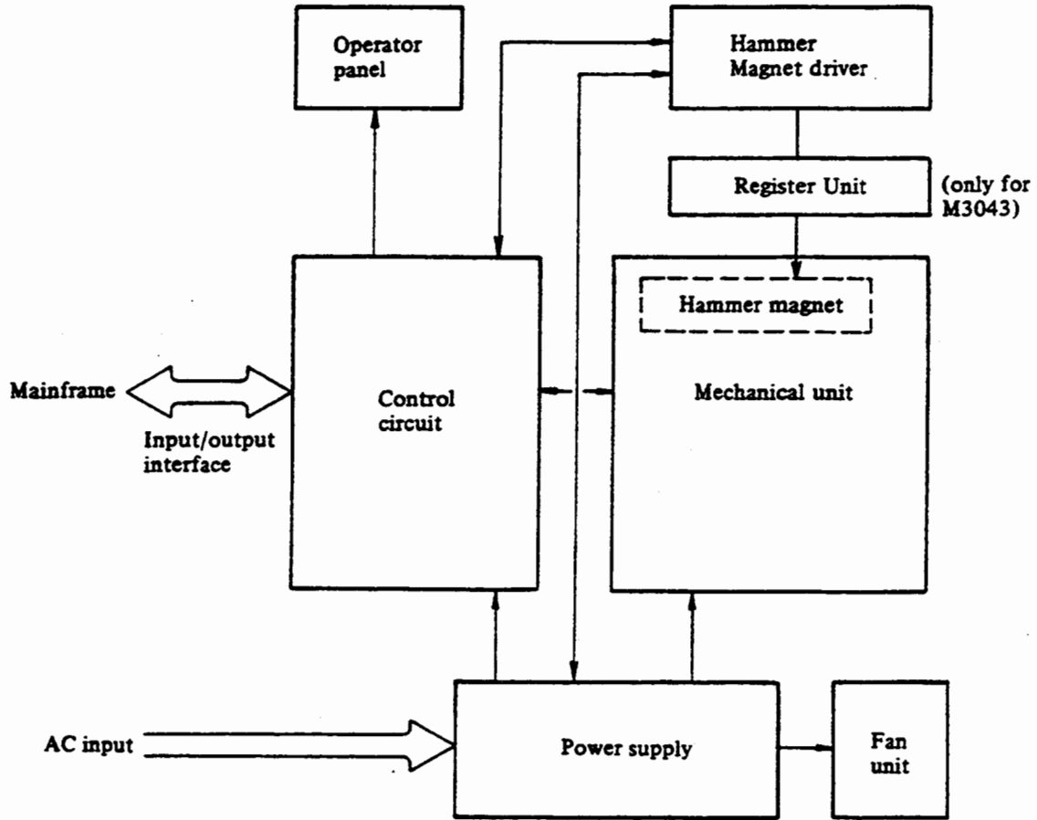
Figure 3.2 Control unit
