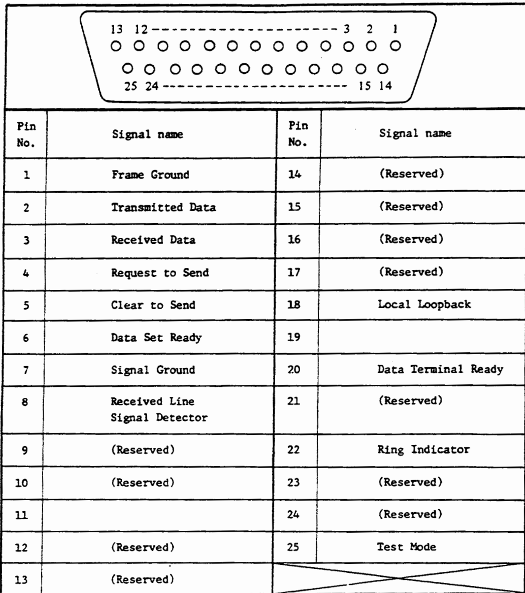
Figure 6.10 RS-232-C interface connector pin assignment
