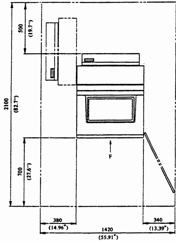
Maintenance area for M3043
