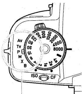
Set to "P".
